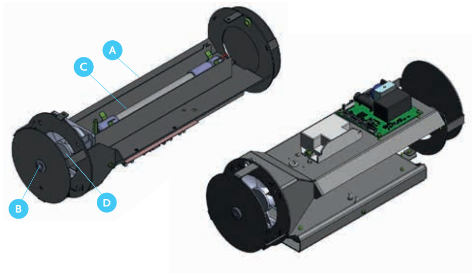
A Case · B On/Off button with blue control light · C UV-C special bulb · D Fan
